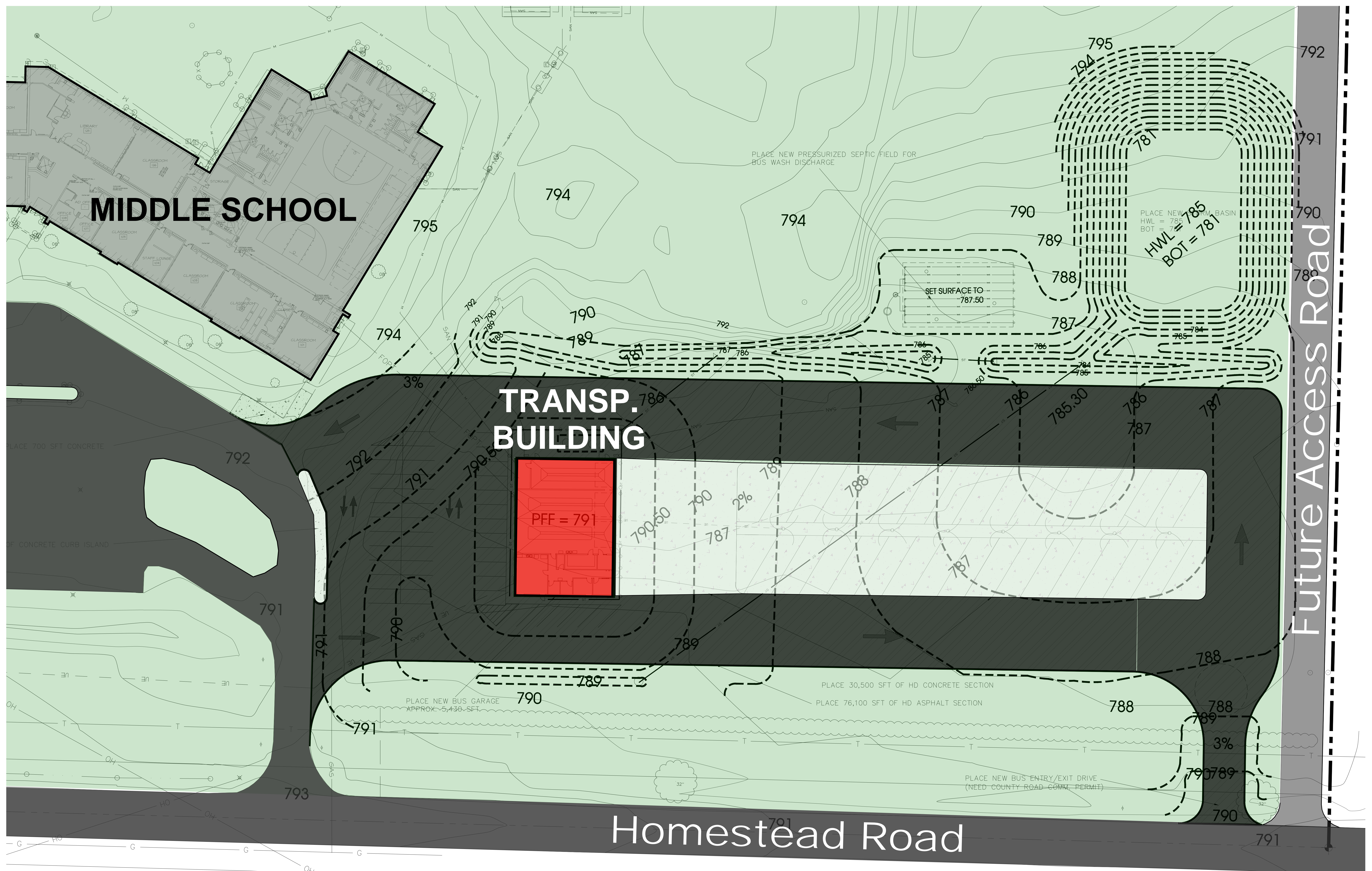
Site Plan
